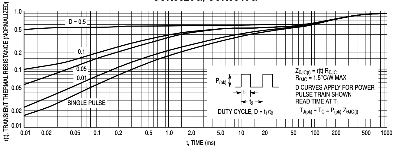
Figure 17. Thermal Response
